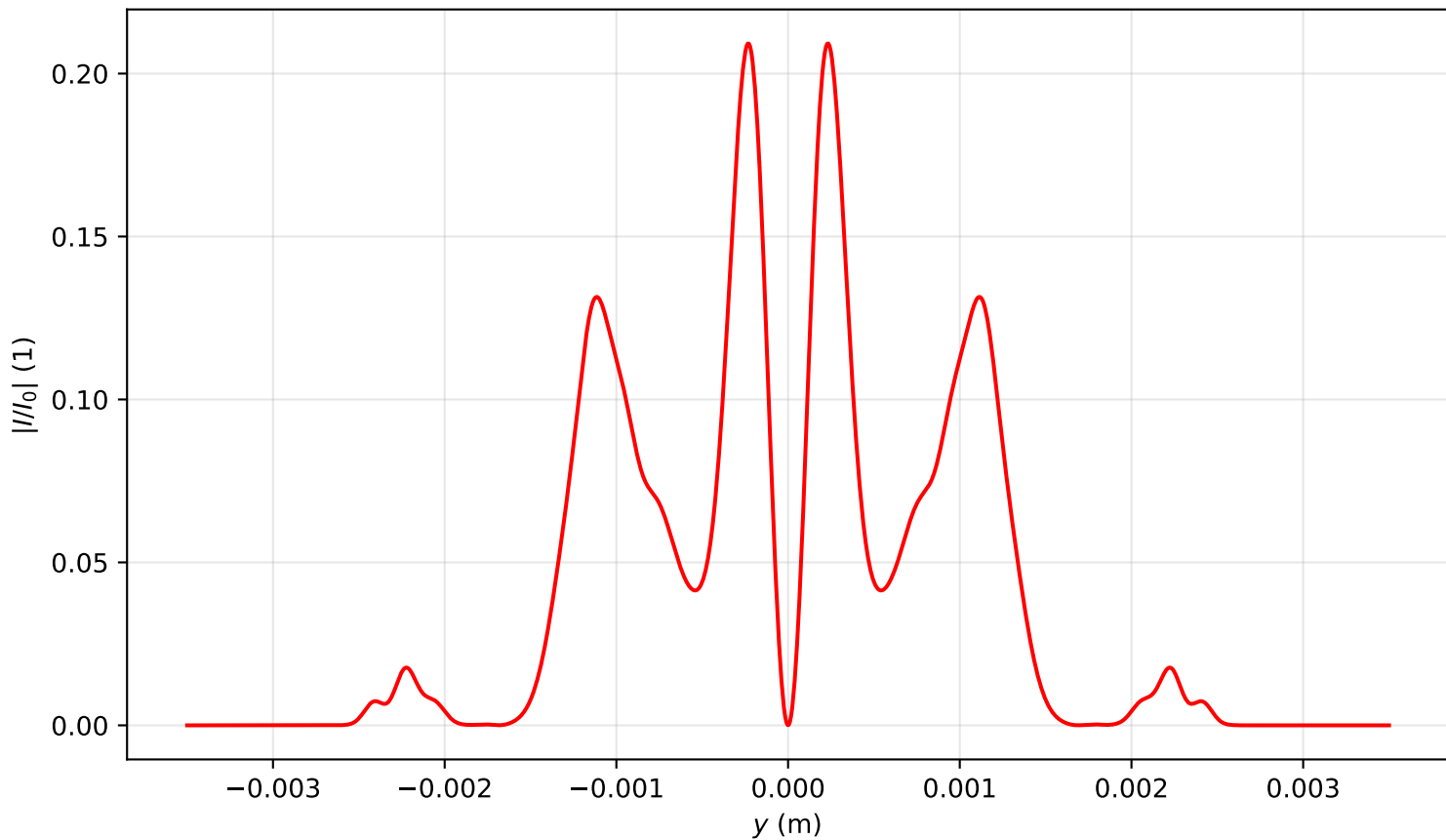
Intensity profile I(x = 0, y, z = 1.831)/I_0 , \text{Pin}=9.0\text{Pcr} , artificial time
